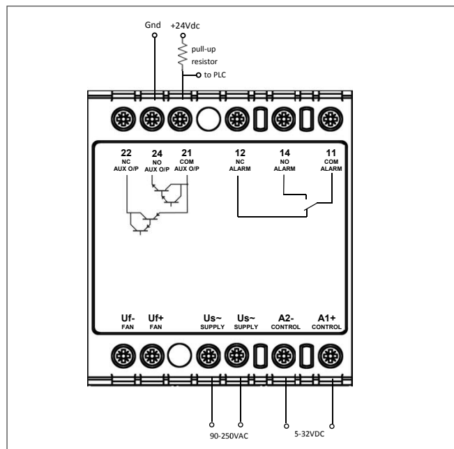
Connection of normally open auxiliary output (24-21) in an 'nnp' style
